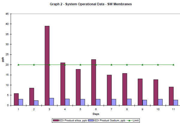
GRAPH 2, SYSTEM DATA – SW
