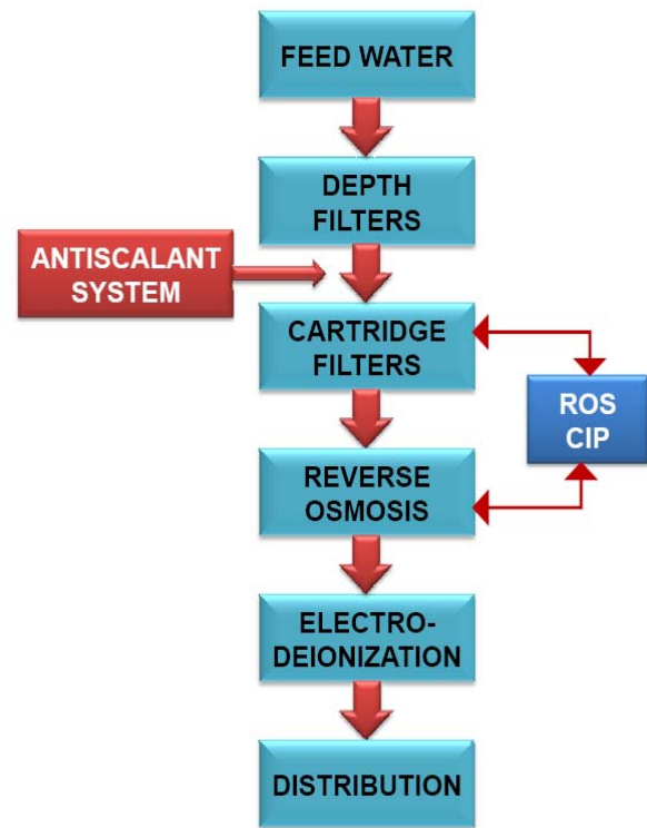
FIGURE 1–WATER TREATMENT SYSTEM
