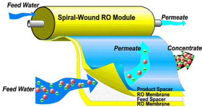
FIGURE 4 - ROS MEMBRANES
