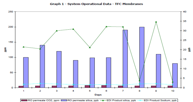
GRAPH 1, SYSTEM DATA TFC
