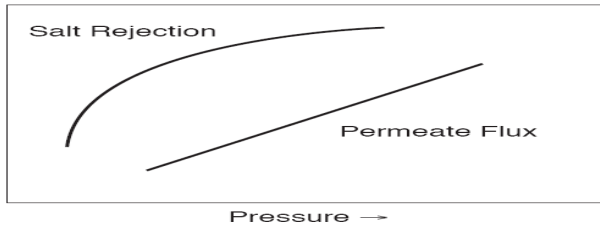
FIGURE 6 – EFFECT OF FEED WATER PRESSURE ON SALT REJECTION & FLUX
