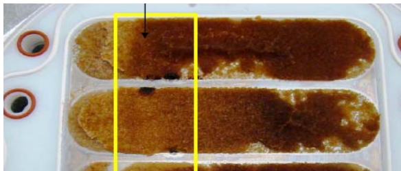
FIGURE 9 – RESIN BURNED EVIDENCE
